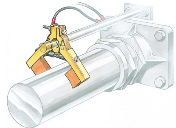
Electro Eliminator Number 2 for 2" - 8" diameter shafts.
